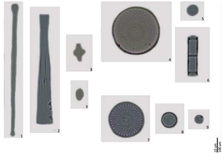
Appendix 1. Selected diatom species used to interpret environmental conditions through time in Shadow Lake.
